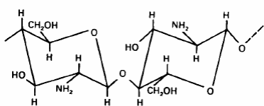
Fig.2. Chitosan Structure
