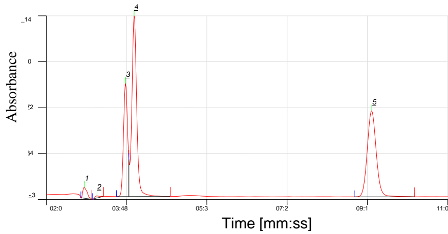
Fig.4. Standard chromatogram of glucosamine for 1 milligram per milliliter solution
