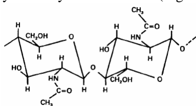
Fig.1. Chitin Structure
