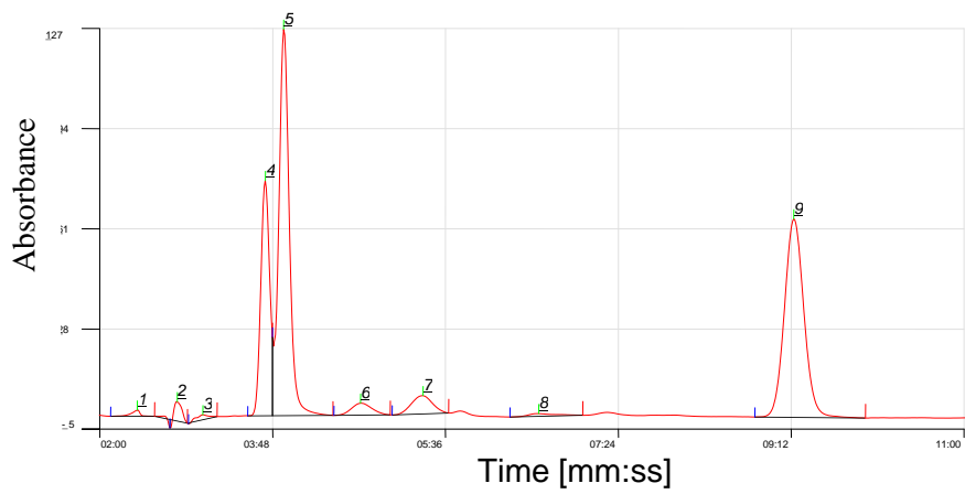
Fig.5. Chromatogram of hydrolyzed chitosan of sample 1 with concentration of 20 milligram of raw material in 15 ml of acidic solution.
