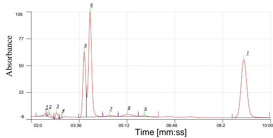
Fig.6. Chromatogram of hydrolyzed material in sample 2 with concentration of 20 milligram of raw material in 20 ml of acidic solution.
